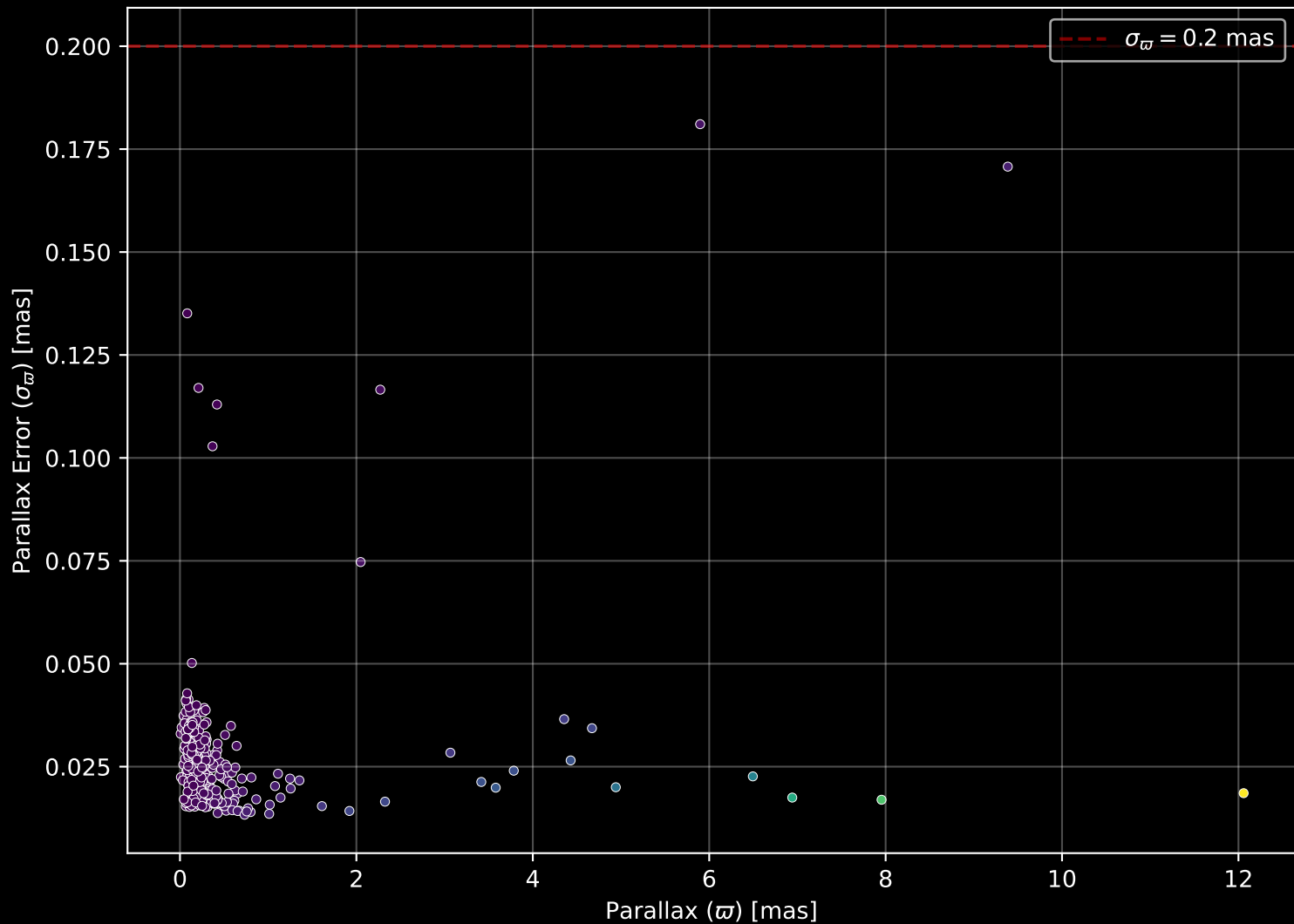
APOGEE DR17 Field: [350+12] Parallax Quality (n= 390)
