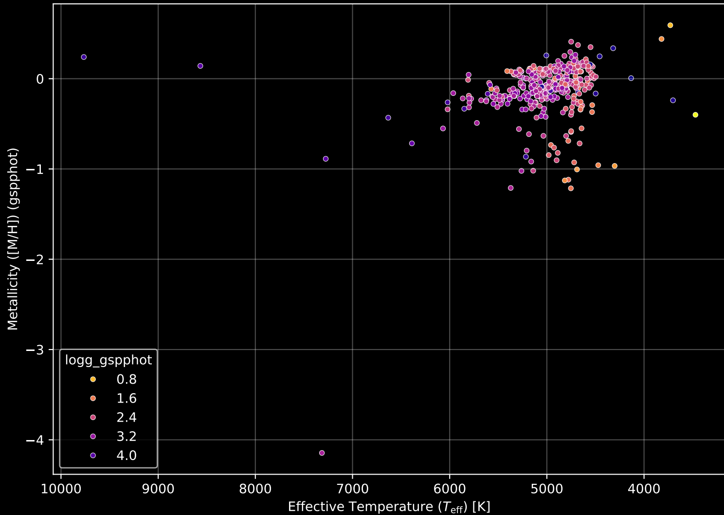
APOGEE DR17 Field: [350+12] Stellar Population Parameters (n= 390)
