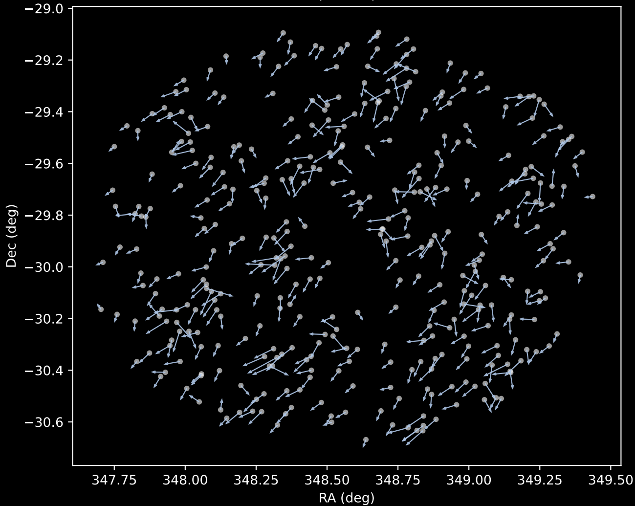
APOGEE DR17 Cluster 1 Proper Motion Vectors (n=377)
