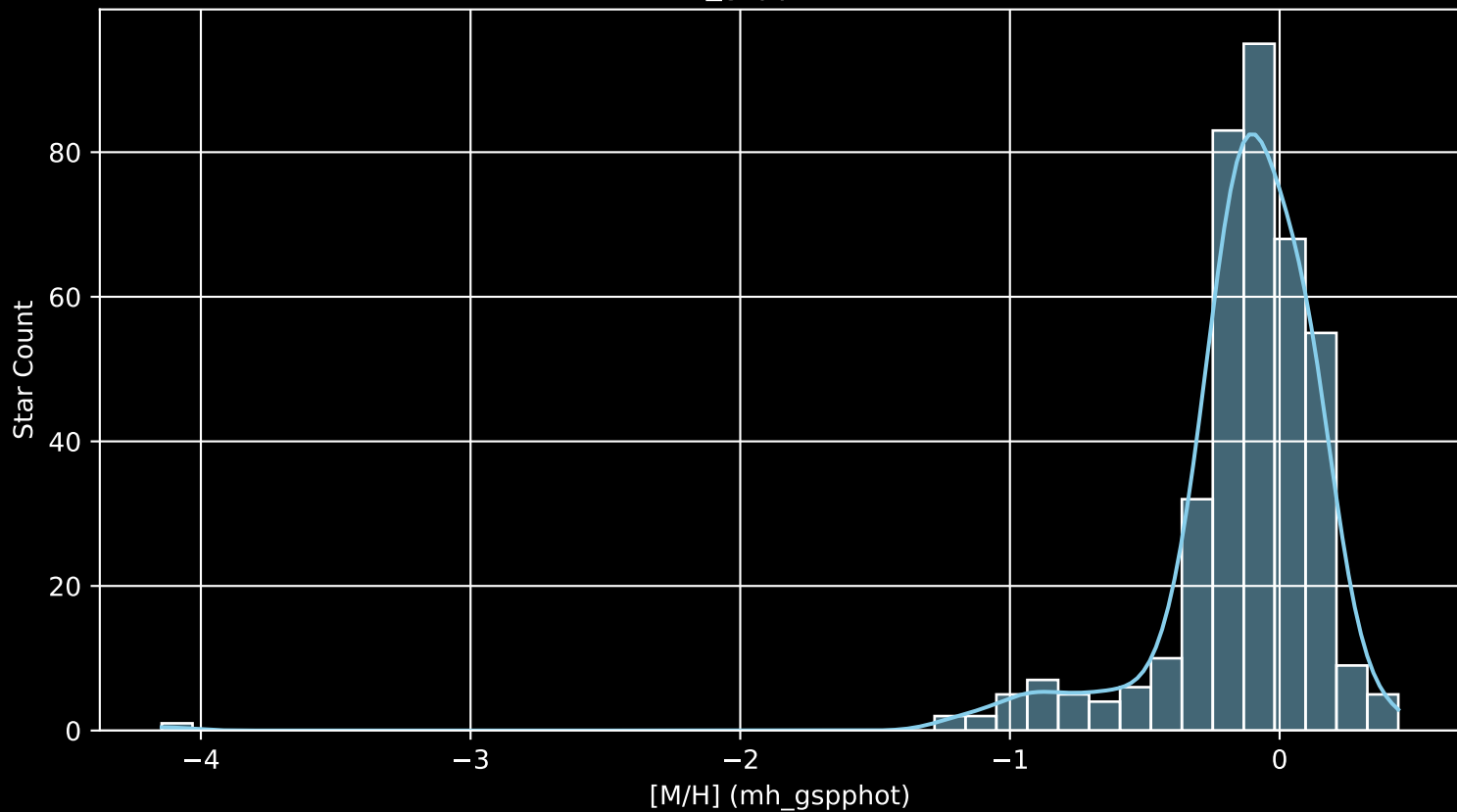
APOGEE DR17 Field: [350+12 [M/H] (mh_gspphot) (n= 389)
