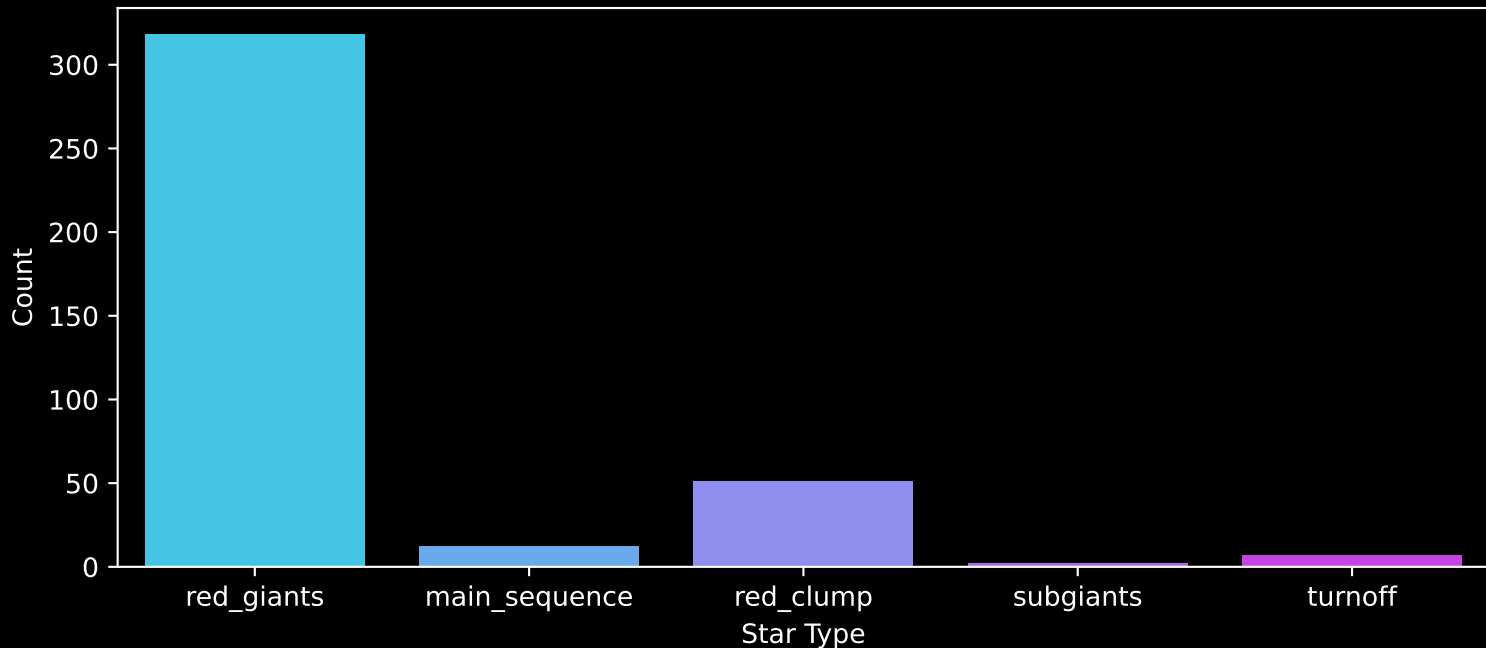
APOGEE DR17 Field: [350+12] Count plot of Star Type
