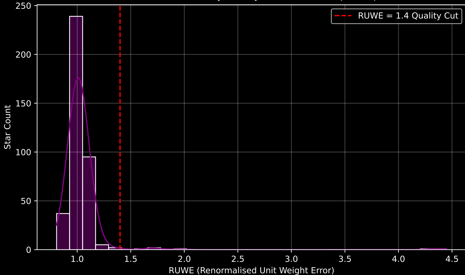
GAPOGEE DR17 Field [350+12] RUWE Distribution (n= 384)
