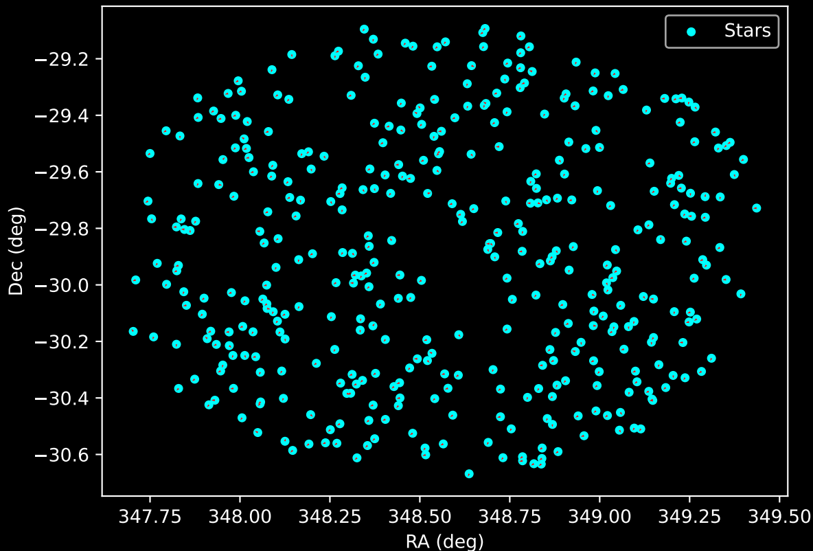
APOGEE DR17 Field: [350+12] Proper Motion Vectors for Gaia Star Field (n= 390)
