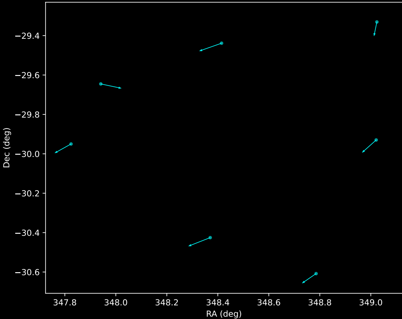
APOGEE DR17 Noise Stream Proper Motion Vectors (n=7)
