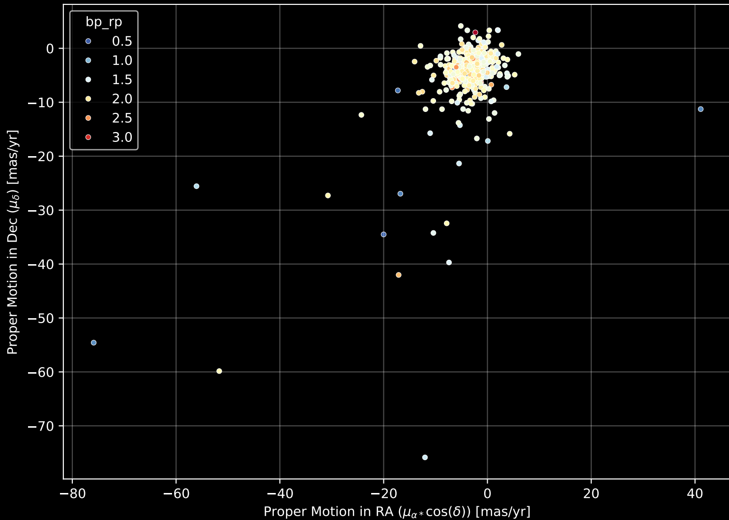
APOGEE DR17 Field: [350+12] Proper Motion Diagram (n= 390)
